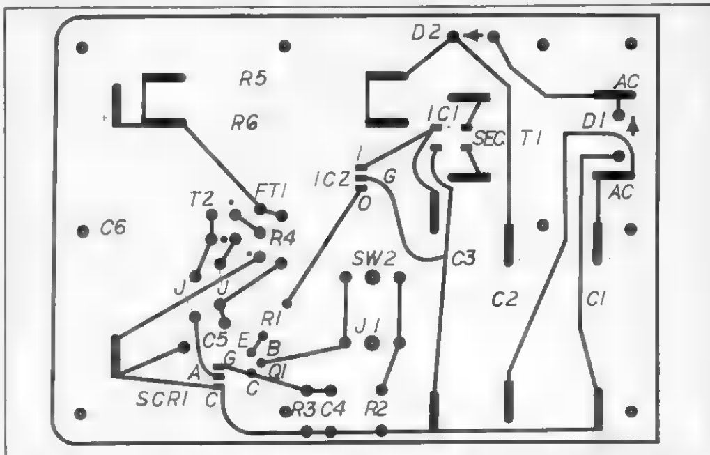
This is the PC pattern and parts placement diagram, shown actual. Use this pattern to make your PC board. Refer to CINEMAGIC #13, 29 if you're not familiar with the procedure for etching a PC board. Drill only the dots with the white dots in the center. Make absolutely sure that all parts properly place before plugging this unit in. Make especially sure that C-1, C-2 and C-6 are correctly installed because these parts could explode if improperly installed.
